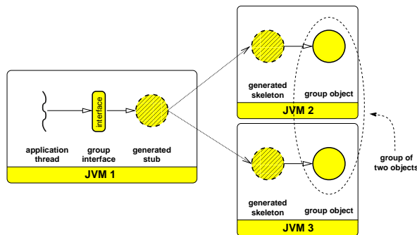
Figure 1: A group invocation with GMI.
