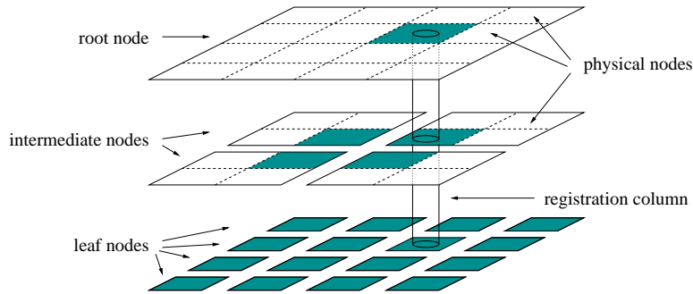
Figure 8: Pyramid for one object handle in a partitioned tree
