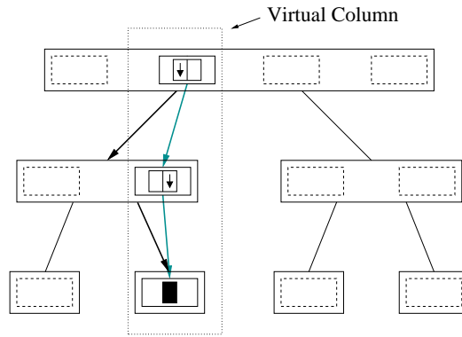
Figure 6: Column for one object handle in a partitioned tree
