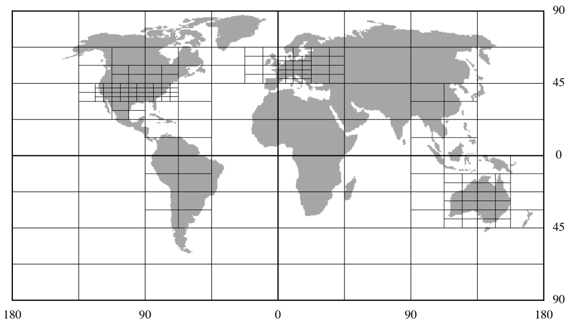
Figure 10: Quadtree covering the earth's surface
