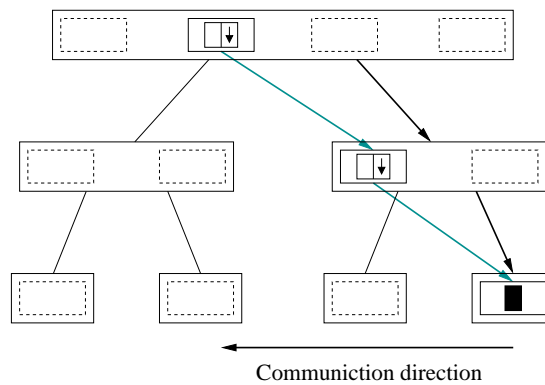
Figure 7: Communication direction while going up in the tree
