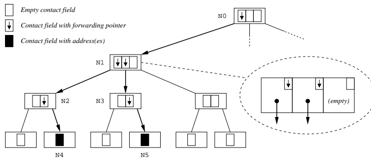
Figure 3: Example: search tree for one distributed object
