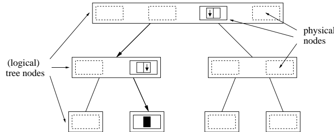
Figure 4: Tree with contact records of one specific object handle
