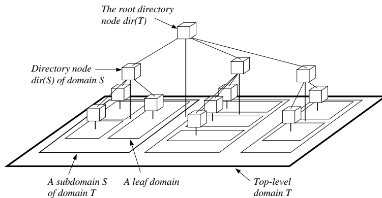
Figure 2: Hierarchical network partition
