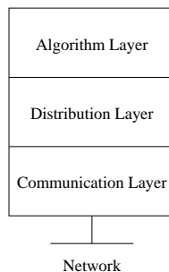
Figure 9: Layering in a physical node
