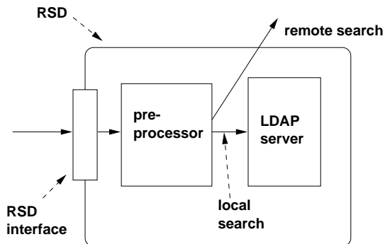
Figure 6: The RSD with preprocessor and LDAP server
