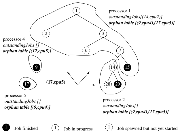
Fig. 1. Orphan saving re-using orphan results.
