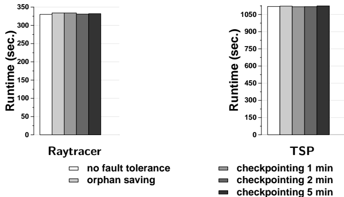
Fig. 2. Application overhead during crash-free execution.
