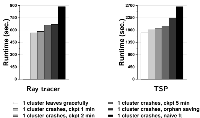
Fig. 3. Application performance in the presence of crashes.
