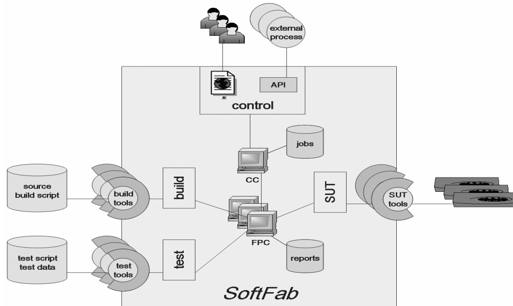
Figure 1. SoftFab architecture
