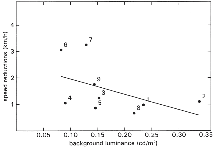
Figure 3. Speed reduction induced by glare source as a function of background luminance.
