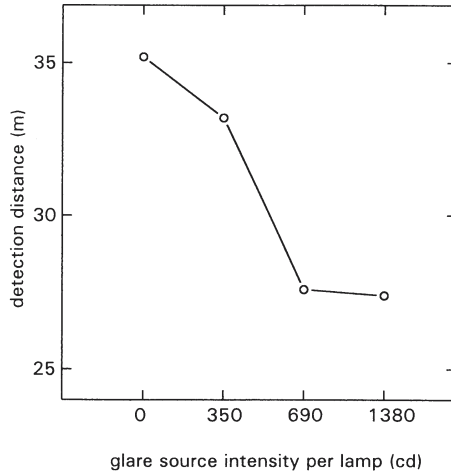
Figure 4. Detection distance as a function of glare source intensity
