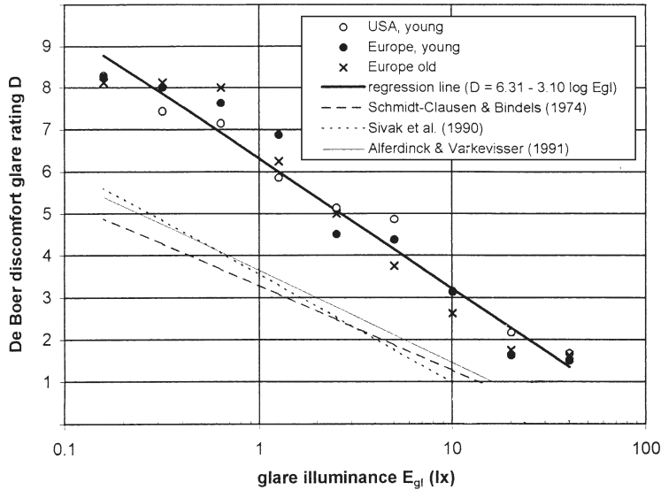
Figure 2. The DeBoer rating as a function of the glare illuminance on the eye of the observer. Also plotted are predictions from the model of Schmidt-Clausen and Bindels (1974), Sivak et al. (1990), and Alferdinck and Varkevisser (1991). The DeBoer scale runs from unbearable (1), disturbing (3), just admissible (5), satisfactory (7), to unnoticeable (9).
