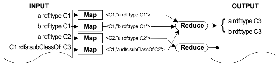
Figure 2: Encoding RDFS rule 9 in MapReduce.
