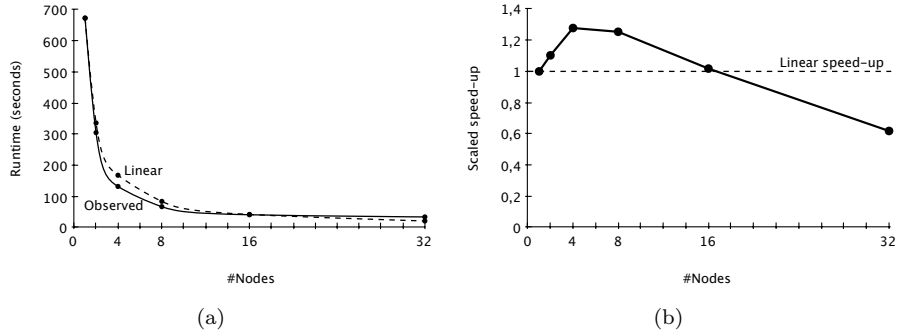
Figure 6: (a) Runtime for the number of nodes (lower is better) (b) Scaled speed-up (higher is better)
