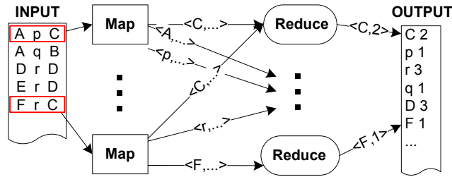
Figure 1: MapReduce processing
