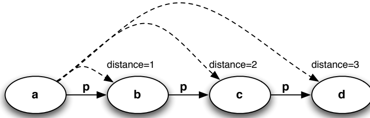
Figure 4: OWL transitive closure
