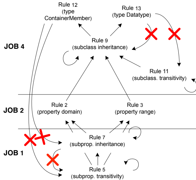
Figure 3: Relation between the various RDFS rules. The red cross indicates the relations that we do not consider.
