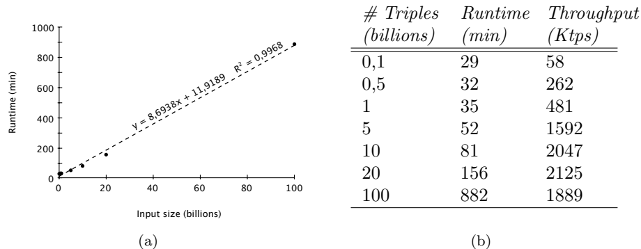
Figure 7: Runtime for increasing input size (on 64 nodes)
