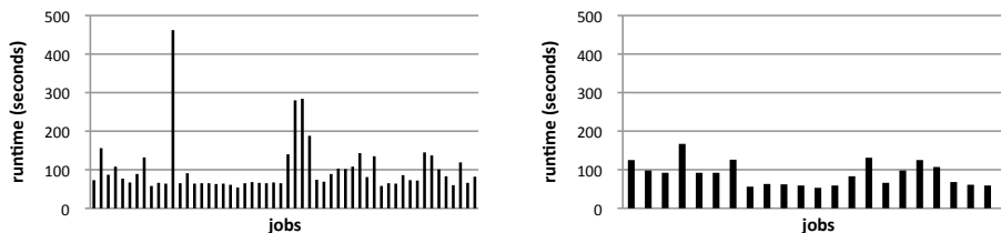
Figure 5: Runtime per job for LDSR (left) and LUBM (right)
