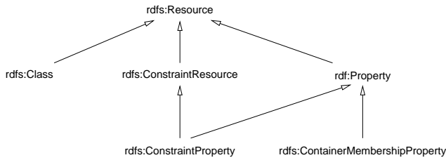
Figure 1: The subclass-of hierarchy of modeling primitives in RDFS.
