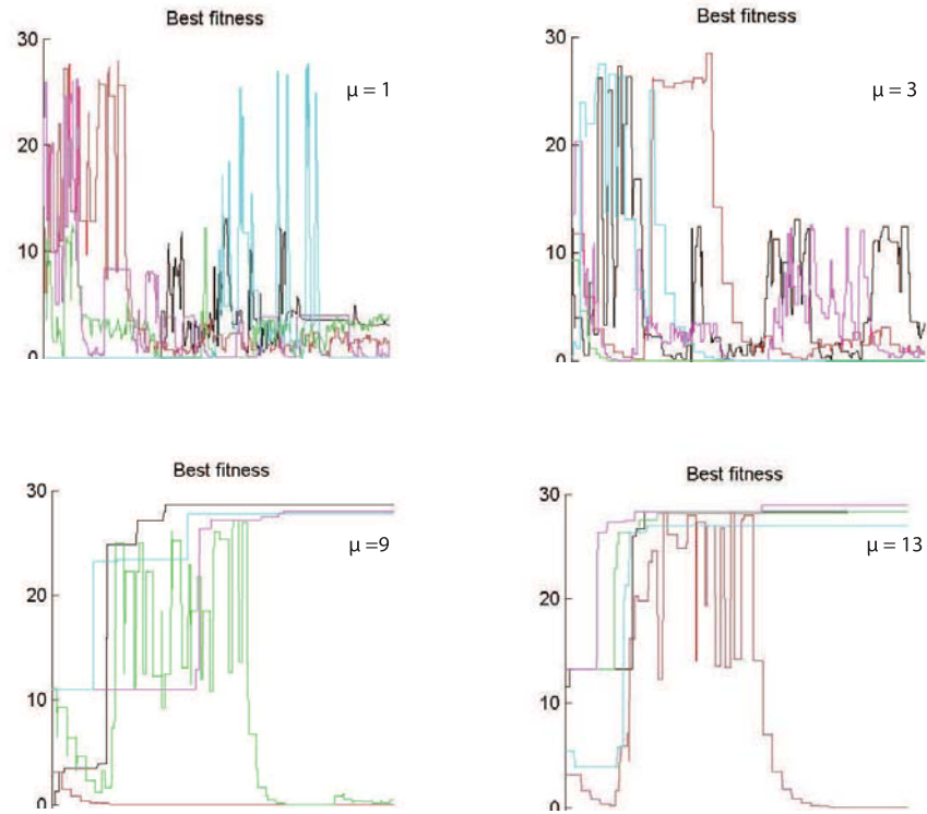
Fig. 5.22 Typical runs for \mu = 1, 3, 9, 13 . The y-axis shows the performance of the current champion, the y-axis the number of generations. Each graph shows five plots; one for each of the five robots in the arena.
