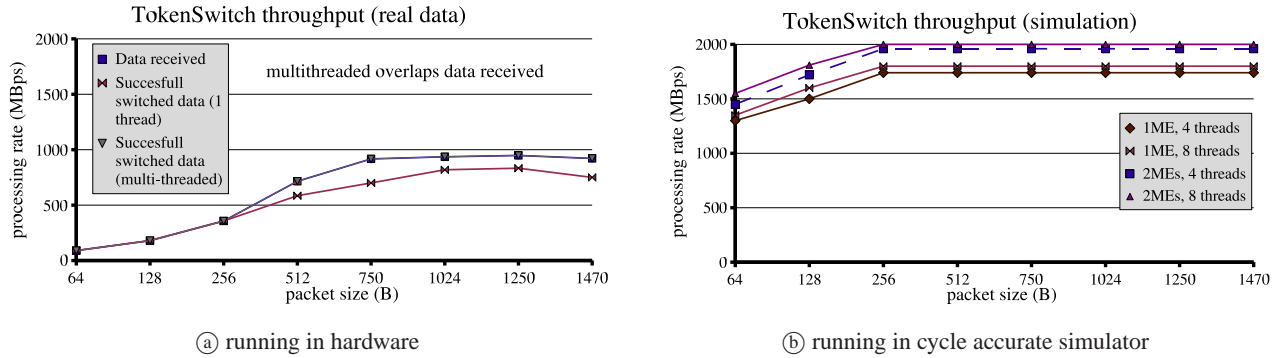
Fig. 7 Token Based Switch performances
