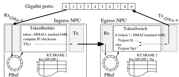
Fig. 5 Token Based Switch using a dual IXP2850.
