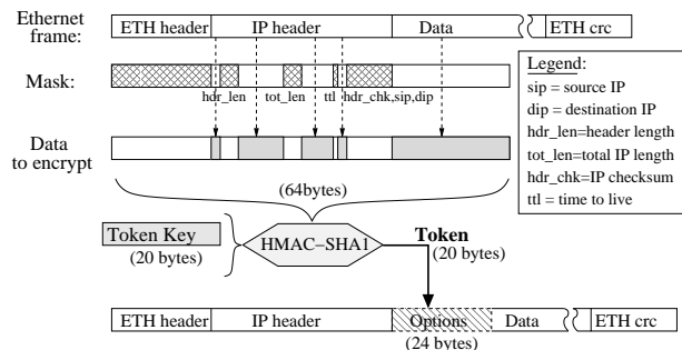
Fig. 3 Token creation.
