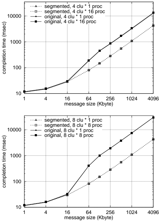
Figure 4. Completion time of MPI_Bcast using 4 clusters (top) and 8 clusters (bottom)
