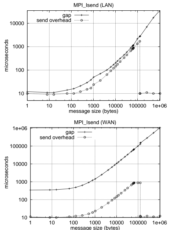
Figure 2. Send overhead and gap for MPI_Isend , measured on the Myrinet LAN (top) and an emulated WAN (bottom)
