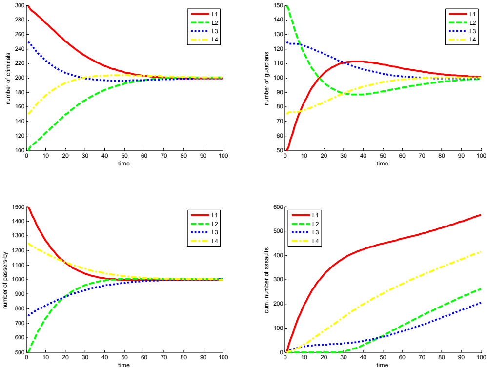
Figure 2. Population-based model - simulation results with complex function
