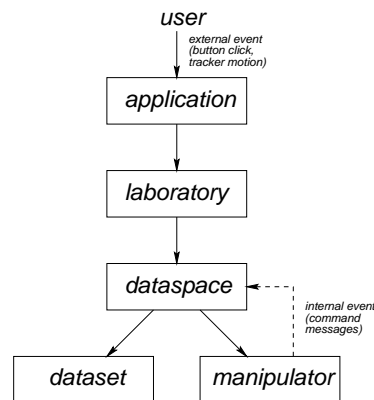
Fig. 3. An example event tree for a simple virtual experiment.
