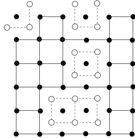
Fig. 1. Some configurations of isolated nodes in the random grid G_n . Dual paths are indicated with a dashed line.
