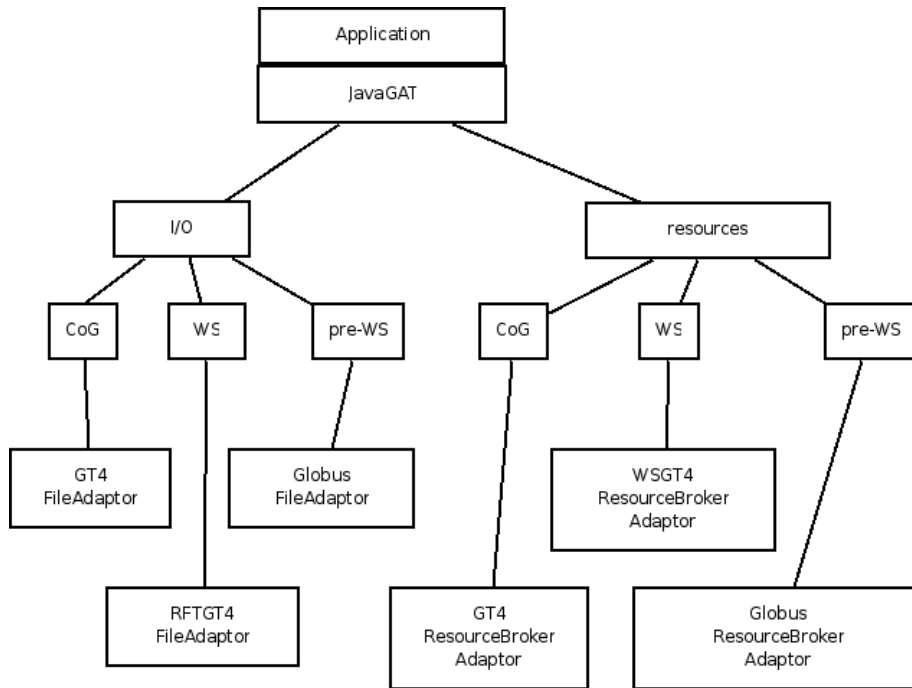
Figure 7.1: Adaptors in JavaGAT
