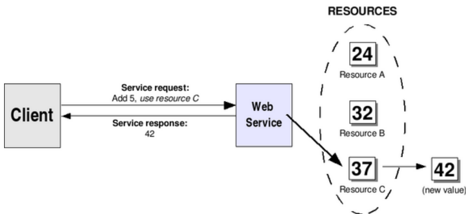
Figure 3.2: Stateful accumulator service
