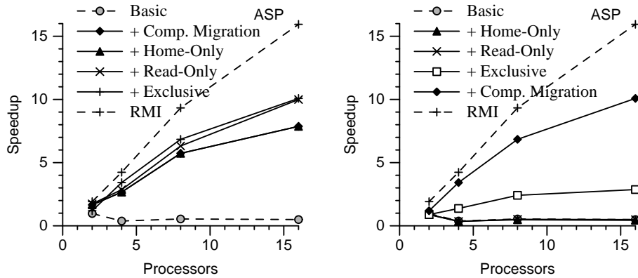
Figure 6: Speedup for ASP. Optimizations are enabled cumulatively, in the legends from top to bottom. Left, the compiler optimization (computation migration) is enabled first, then the RTS optimizations. Right, the RTS optimizations are enabled first, finally the compiler optimization.
