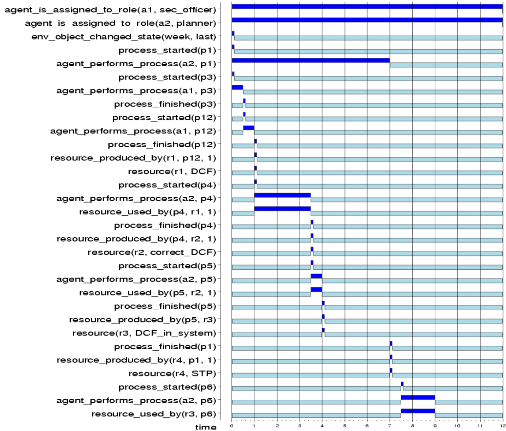
Figure 1 The execution trace used for illustration
