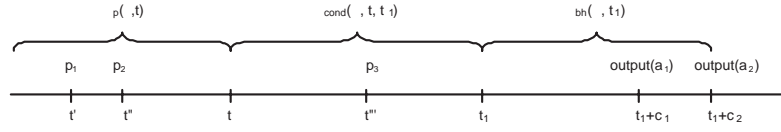
Fig. 3 Graphical illustration of the structure of the past implies future normal form
