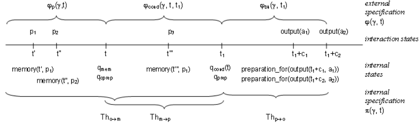
Fig. 4 A graphical representation of relations between interaction states described by a non-executable dynamic property and internal states described by executable rules.
