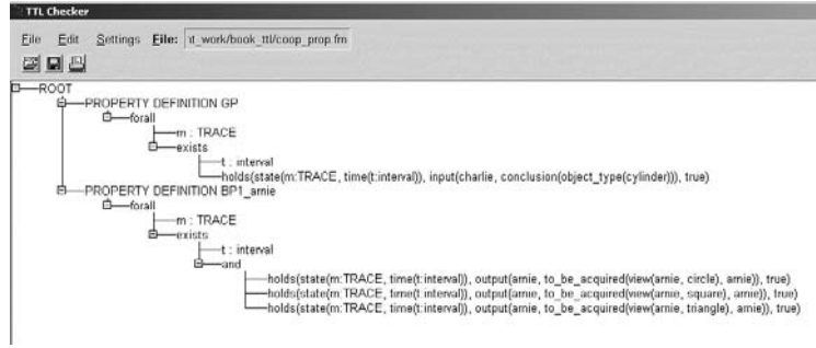
Fig. 5 Screenshot from the TTL Checker Tool
