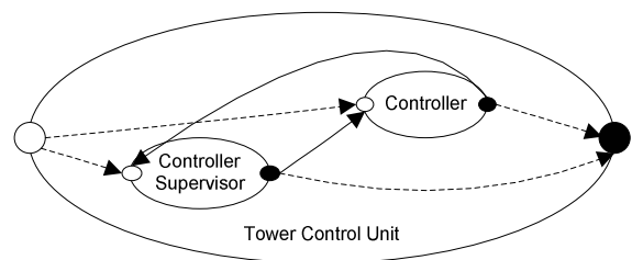
Figure 2. Interaction relations between the subroles of Tower Control Unit role at aggregation level 3
