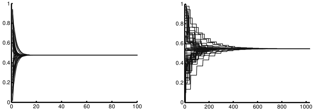
Figure 2. Convergence of the decision states of 50 agents in a group with the parallel (left) and sequential (right) modes of interaction; no external messages are provided to the group. The horizontal axis is time and the vertical axis is the degree of support for the first decision option
