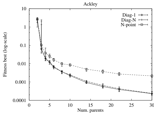
Figure 5. Accuracy curves for the Ackley function
