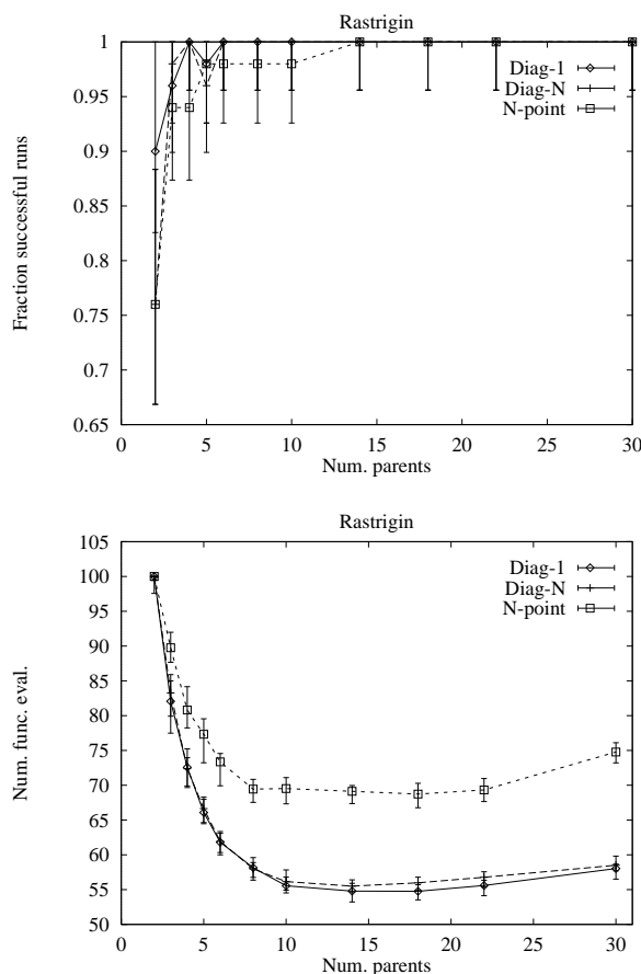
Figure 8. Success rates (upper diagram) and speed (lower diagram) for the Rastrigin function
