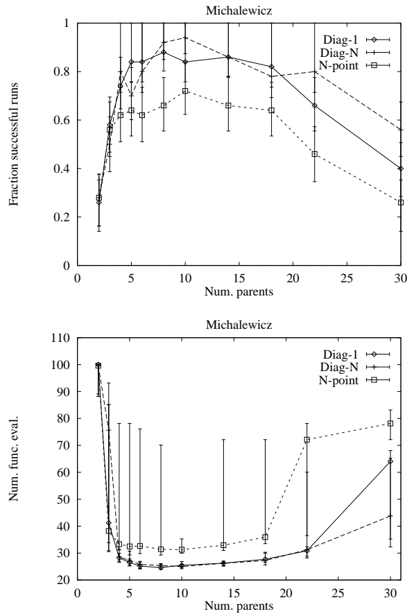
Figure 7. Success rates (upper diagram) and speed (lower diagram) for the Michalewicz function
