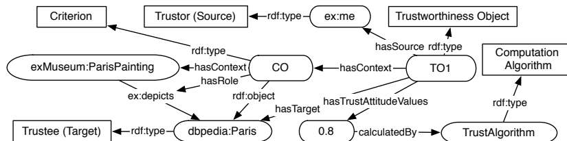
Fig. 2. Snapshot of the trust ontology, specialized for modeling data trustworthiness.
